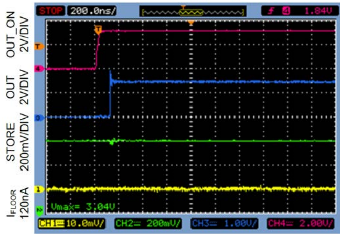
OUT_ON Switched ON : Circuit A with C OUT Removed V IN =1.2V, STORE=3V, I STORE =0.3μA, I OUT =3mA
